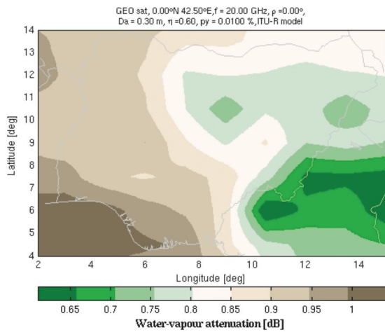
Figure 8: Contour map of water-vapour attenuation for Ka downlink (20 GHz) from NigComsat-1 at 0.01% unavailability.
