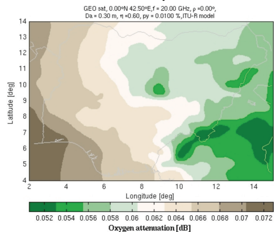
Figure 7: Contour map of oxygen attenuation for Ka downlink (20 GHz) from NigComsat-1 at 0.01% unavailability
