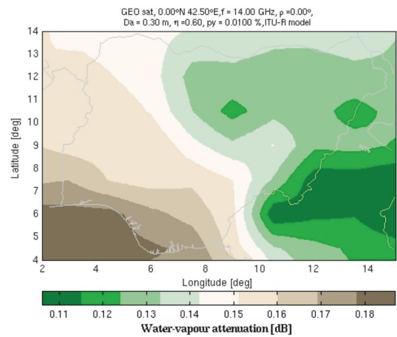
Figure 6: Contour map of water-vapour attenuation for Ku uplink (14 GHz) to NigComsat-1 at 0.01% unavailability.
