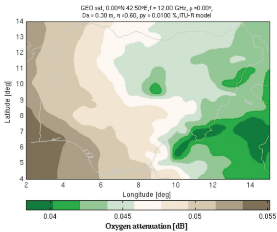
Figure 3: Contour map of oxygen attenuation for Ku downlink (12 GHz) from NigComsat-1 at 0.01% unavailability
