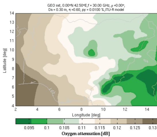
Figure 9: Contour map of oxygen attenuation for Ka uplink (30 GHz) to NigComsat-1 at 0.01% unavailability.
