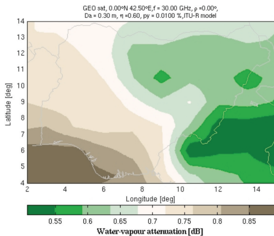
Figure 10: Contour map of water-vapour attenuation for Ka uplink (30 GHz) to NigComsat-1 at 0.01% unavailability.
