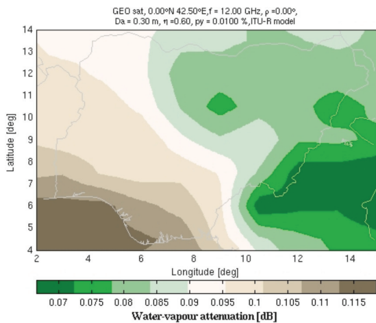
Figure 4: Contour map of water-vapour attenuation for Ku downlink (12 GHz) from NigComsat-1 at 0.01% unavailability
